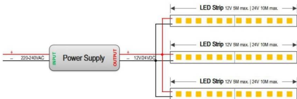
2. How to wire multiple LED strip light:
