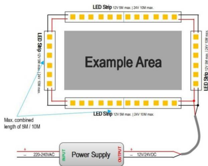
3. Wiring example for projects - 24VDC
