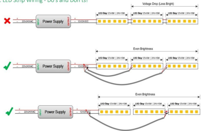
5. LED Strip Wiring - Do's and Don'ts!
