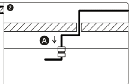
Pass the AC cable through the waterproof connector and tighten it to prevent water.
