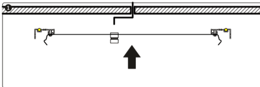
Fixing the ceiling mounted back-plate to the ceiling.
