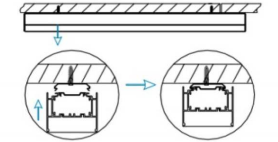
2.Put the snap-fit into the setscrews and lock it tightly.
