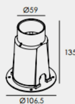
Recessed Sleeve 184#
