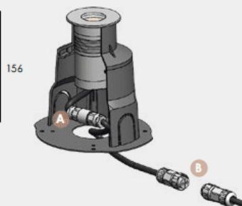
Recessed Sleeve 184#
