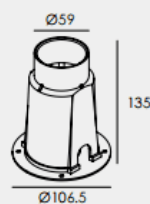
Recessed Sleeve 184#
