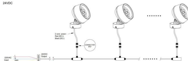
24VDC
