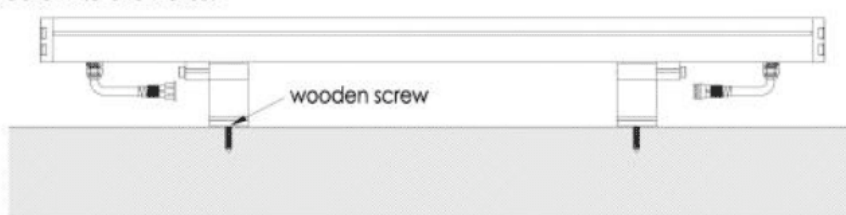
CONNECTOR: IP67
